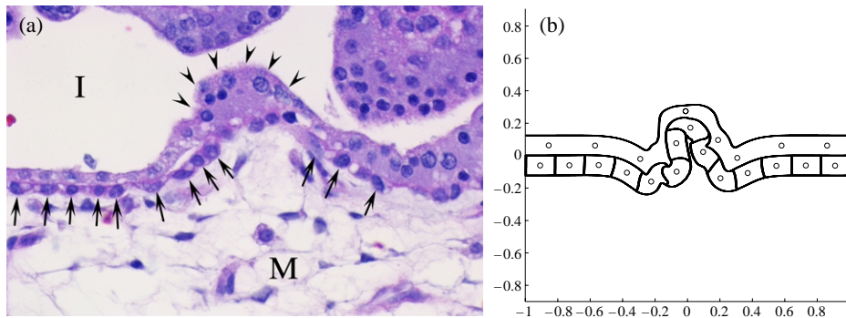
Figure 24. Comparison of in vivo (a) and computer simulated (b) trophoblast evagination. (a) Region of budding (evagination) seen in a first trimester villous. Note continuous layer of CTs in regions on either side of evagination (arrows) and increased amount of cytoplasm and number of nuclei in ST layer in region of evagination (arrow heads). Villous matrix core (M) and intervillous space containing a few maternal erythrocytes (I). (b) Computer simulation of evagination obtained by initiating several cell fusions followed by consecutive proliferations of cells occupying the same small area of the tissue.
